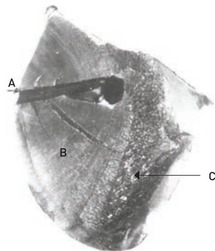
Fatigue fracture surface of a failed gear showing the conchoidal “beach markings” radiating from the oil hole, marked (A). Also shown are the “beach markings” associated with fatigue crack growth (B), and the area where ductile overload occurred (C).
